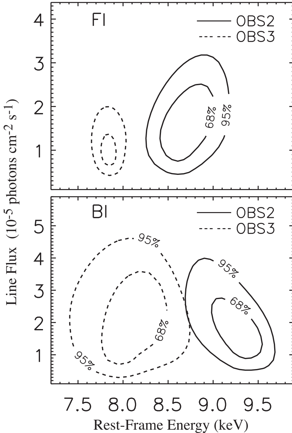
Fig. 2.— 68% and 95% confidence contours of absorption-line fluxes versus absorption-line energies of the first modeled absorption line (model 7, Table 3). The upper and lower panel contours correspond to fits performed to the FI and BI spectra, respectively. Solid and dotted lines are contours for epochs OBS2 and OBS3, respectively.
